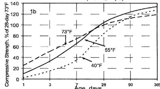
Figure 1 Effect of Temperature on Set Time (1a) and Strength (1b) of Concrete
