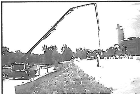
Figure 1: A vertical pump boom configuration can result in loss of entrained air in concrete
